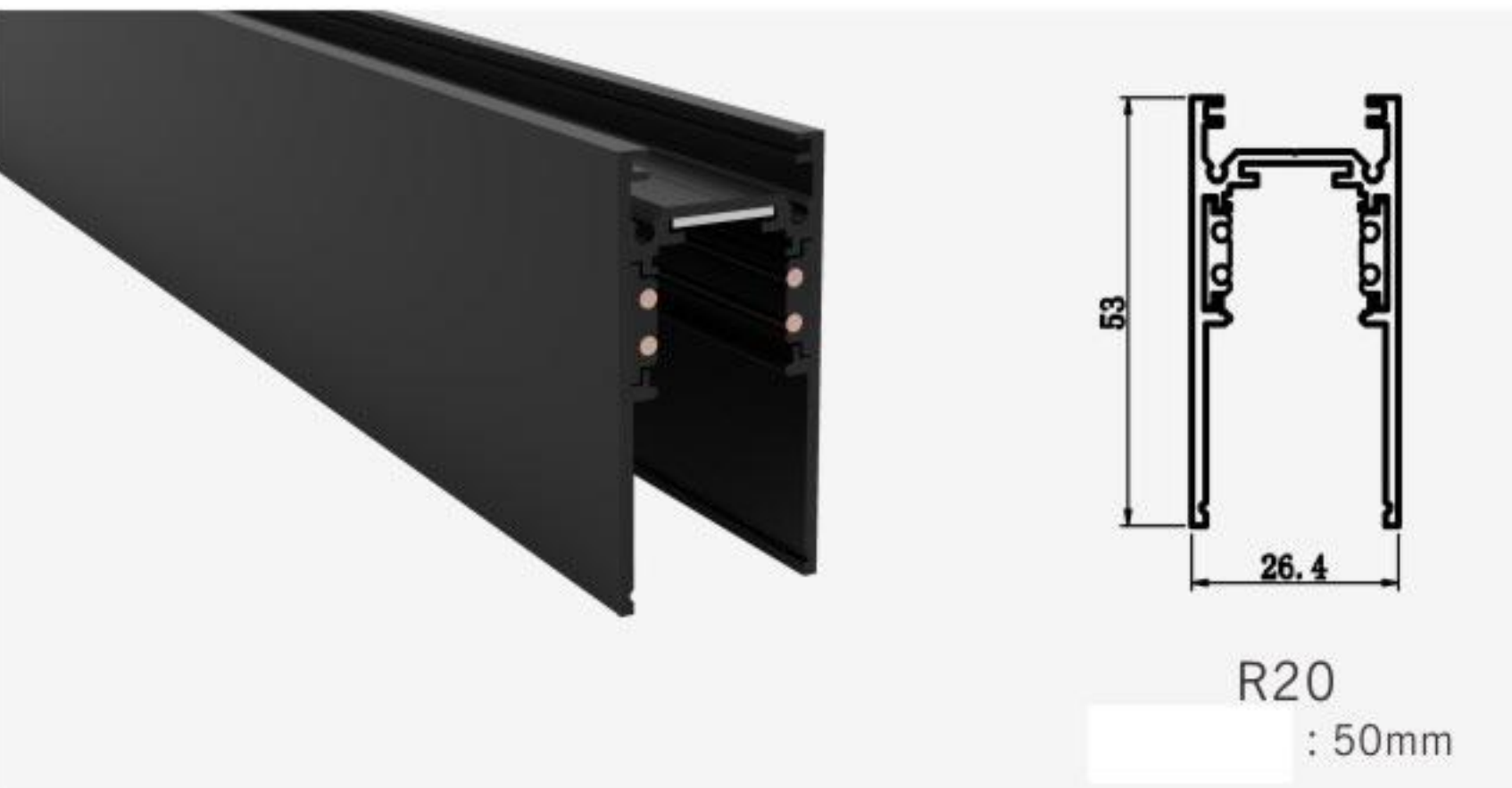
S20 Size : 26.4X78.4X26.4mm
