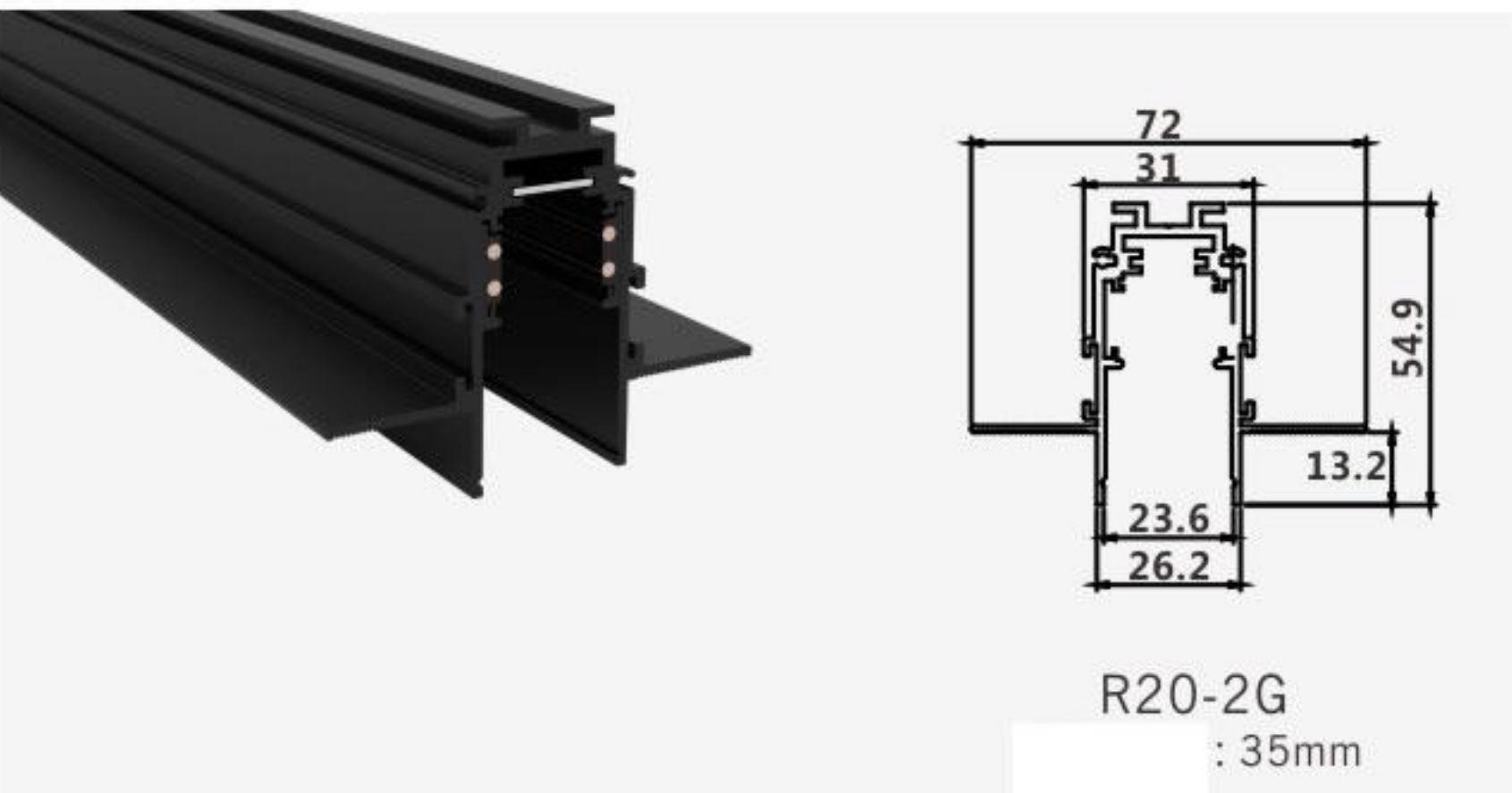
R20-2G Size : 31X53X72mm
