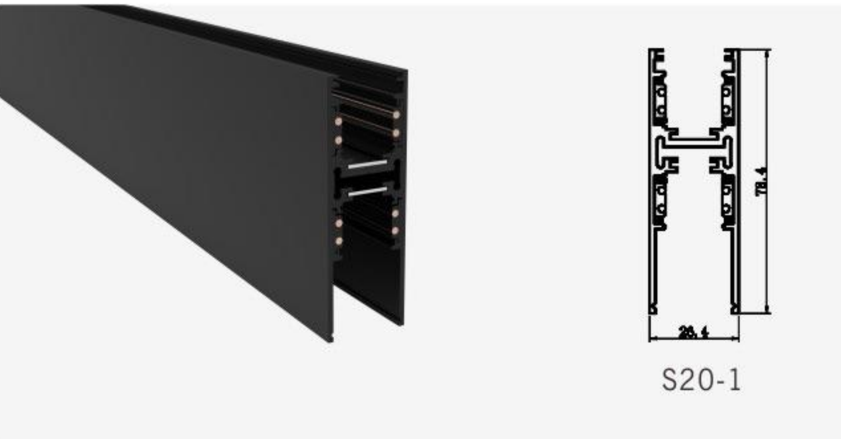
S20-1 Size : 26.4X78.4X26.4mm
