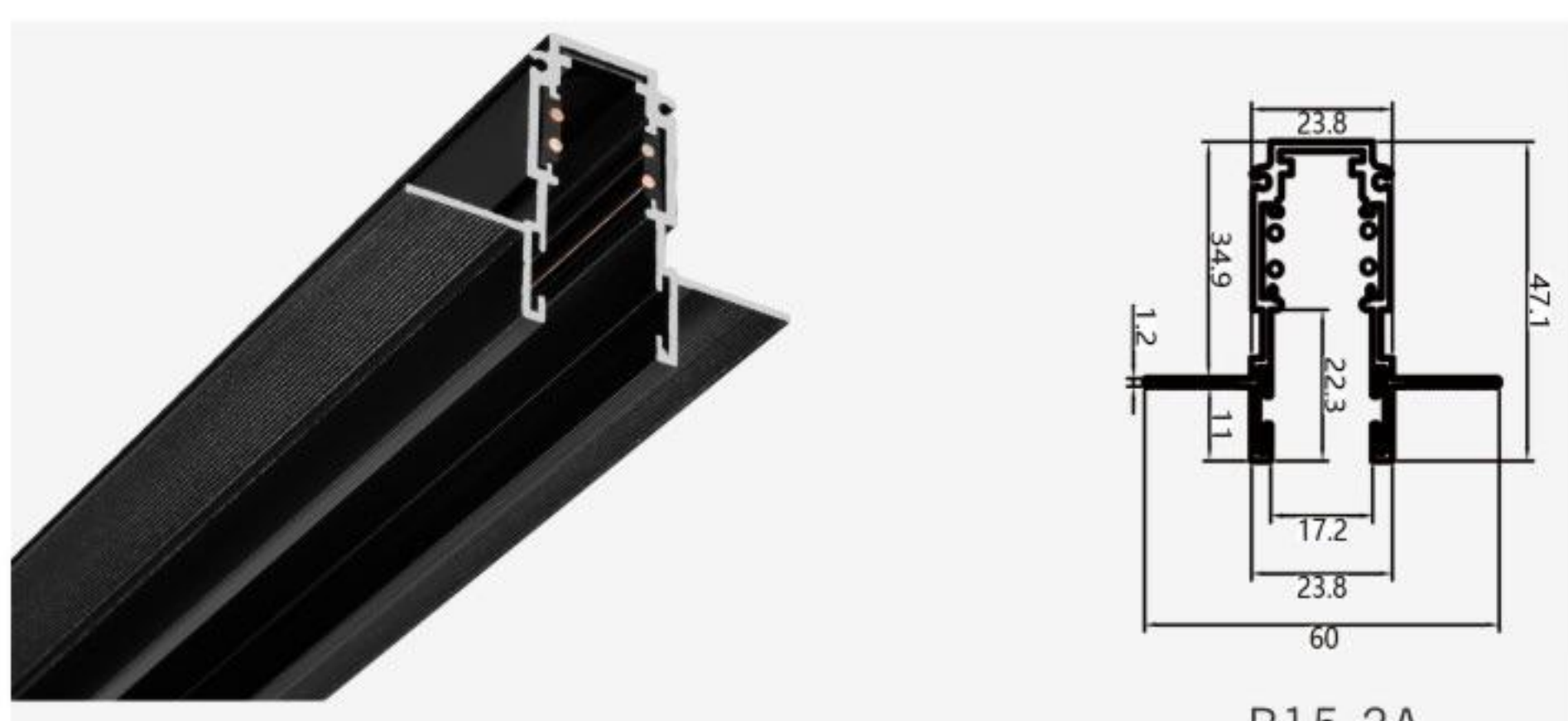
M15-R15-2A Size: L1000*W60*H47.1mm
