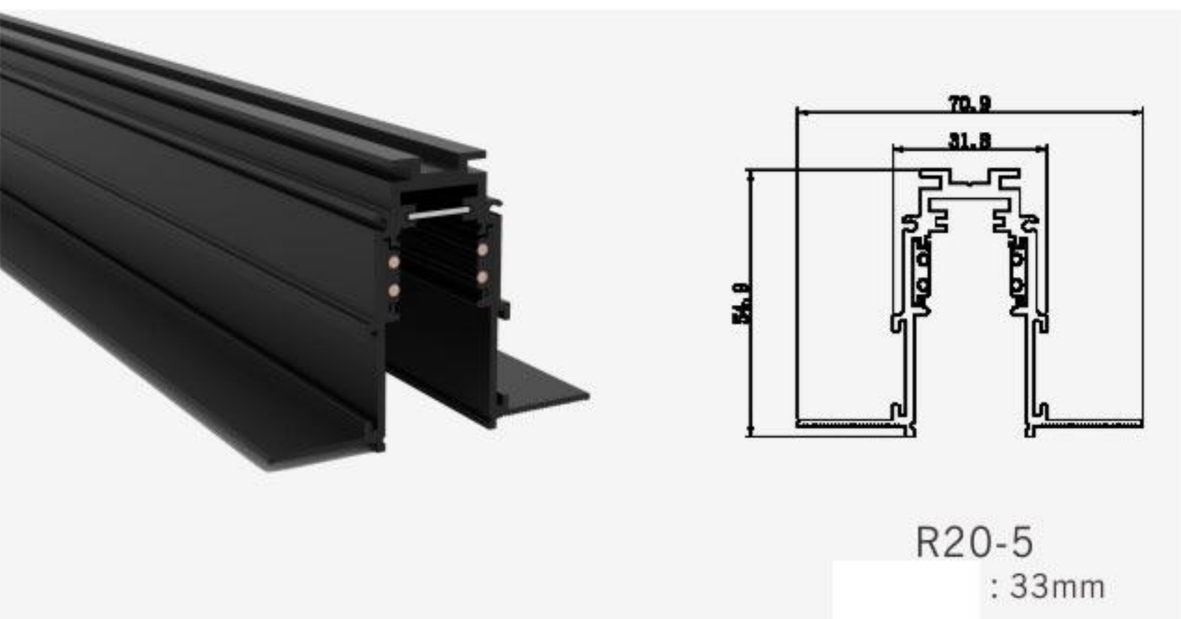
R20-5 Size : 70.9X54.9X31.8mm
