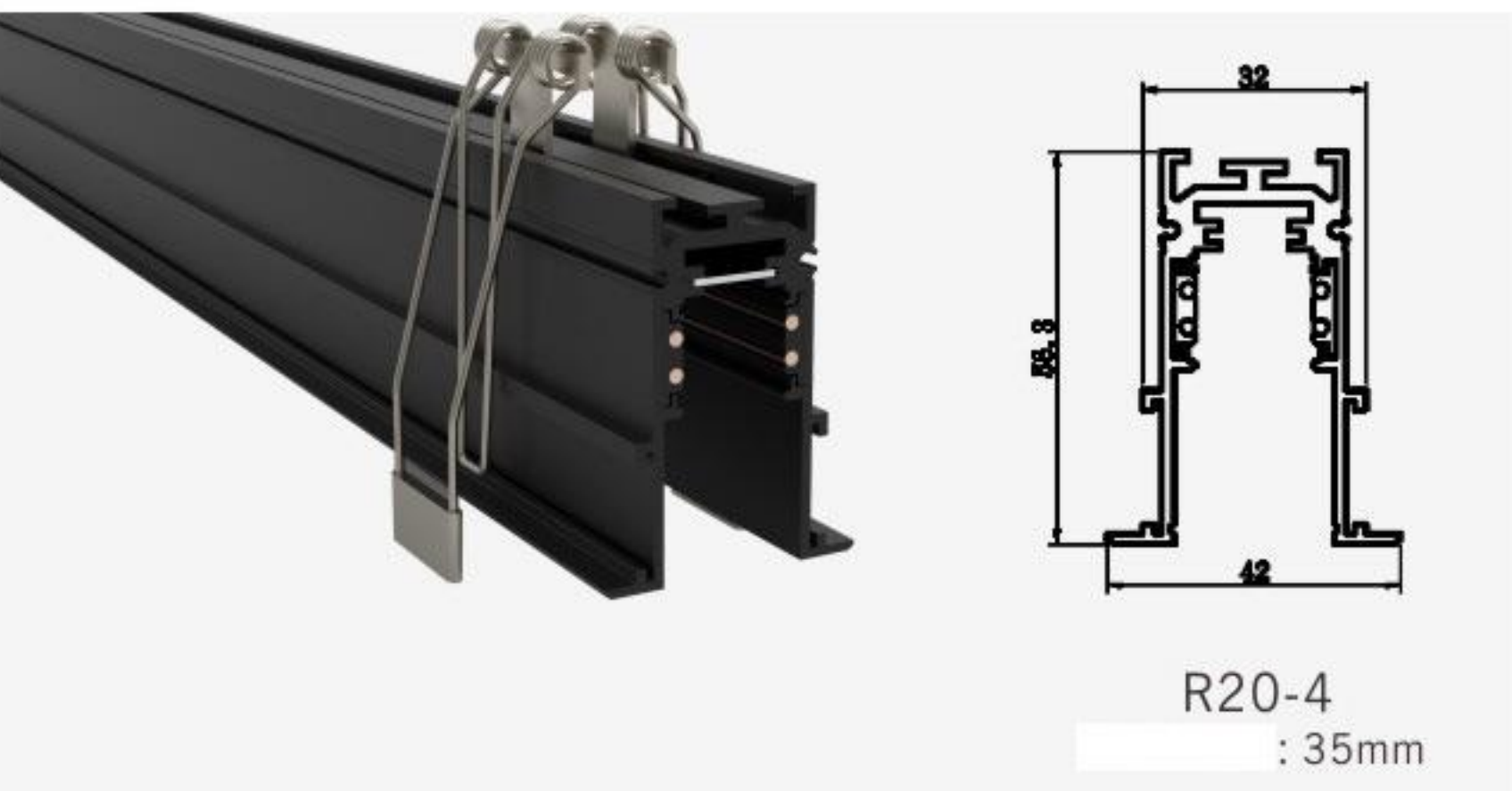
R20-4 Size : 32X56.3X42mm
