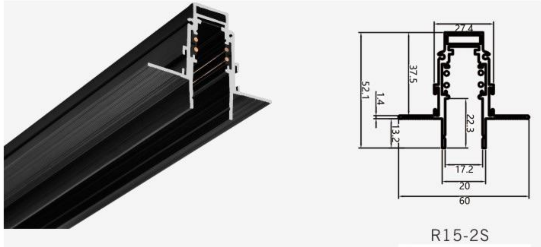
M15-R15-2S Size: L1000*W60*H52.1mm
