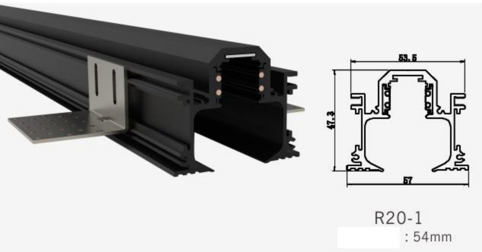
R20-1 Size : 53.5X47.3X57mm
