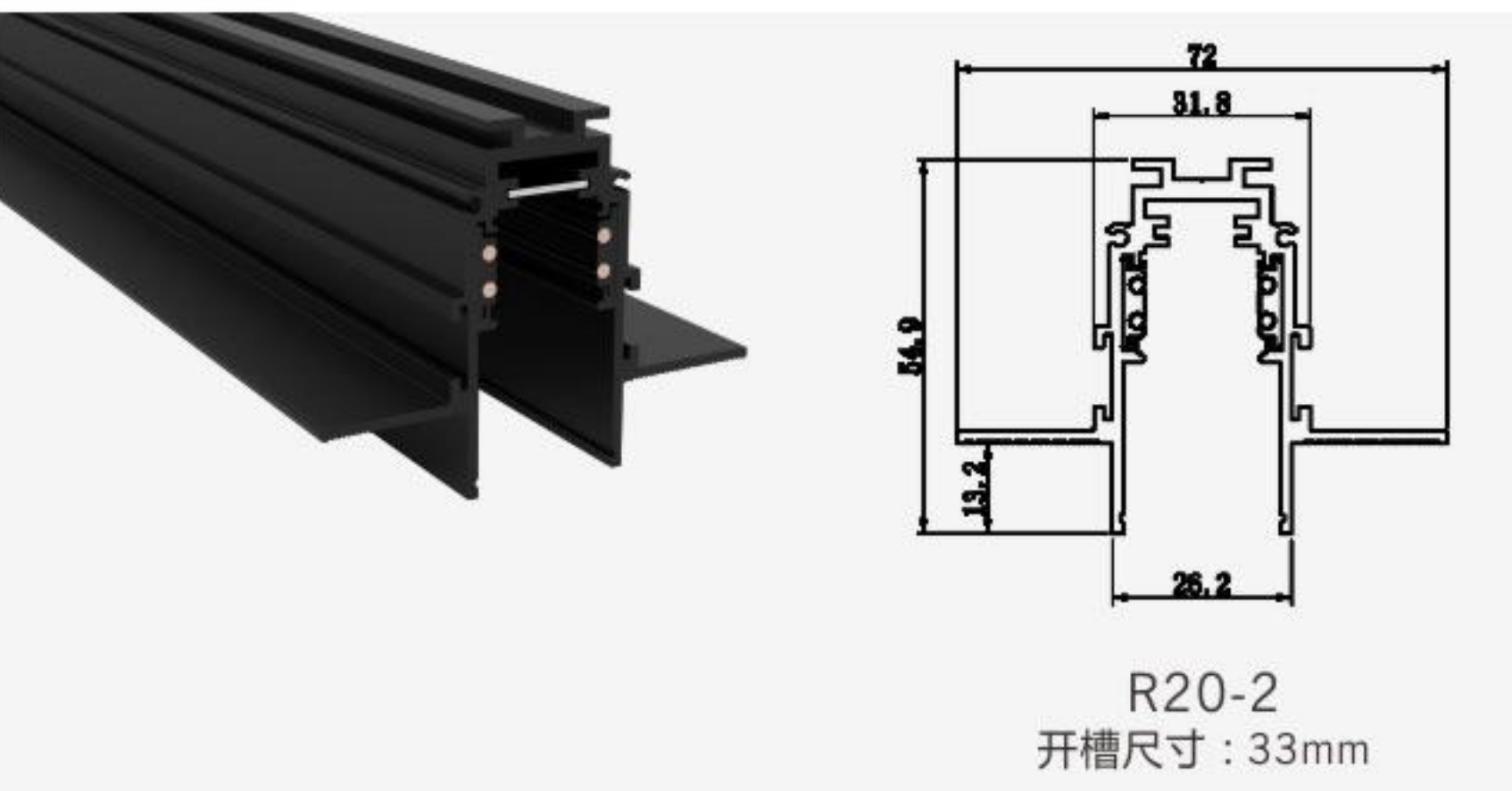
R20-2 Size : 72X54.9X26.3mm
