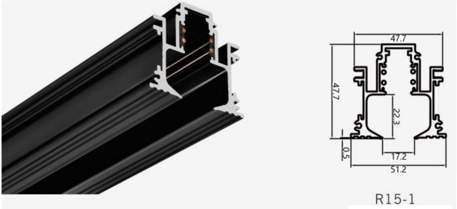
M15-R15-1 Size: L1000*W47.7*H47.7mm
