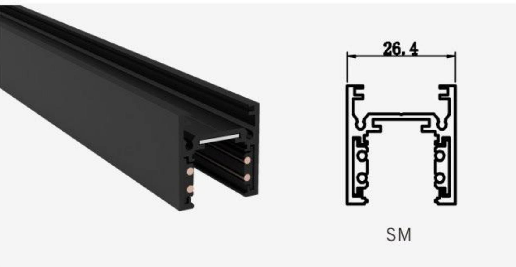
SM Size : 26.4X26.4X26.4mm
