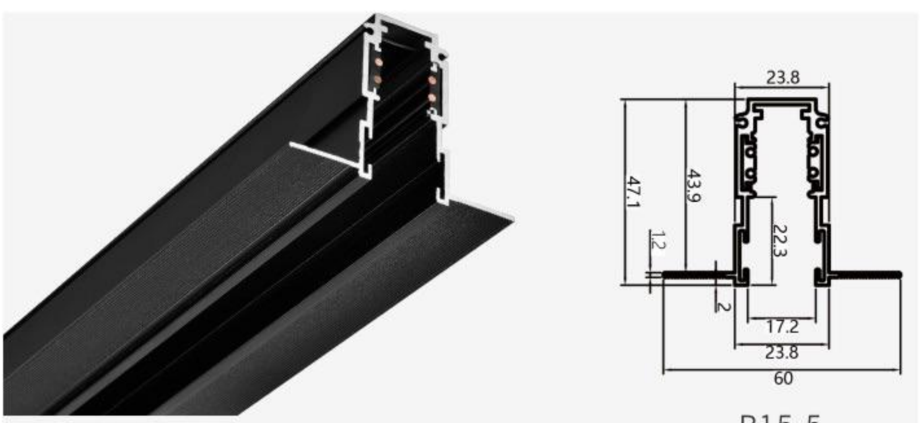
M15-R15-5 Size: L1000*W60*H47.1mm
