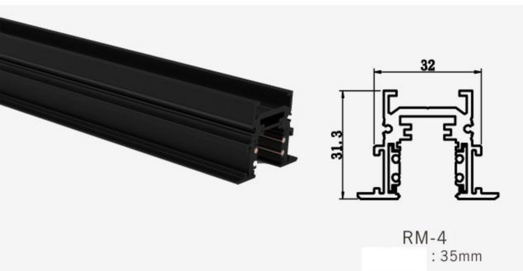
RM-4 Size : 31.3X32X42
