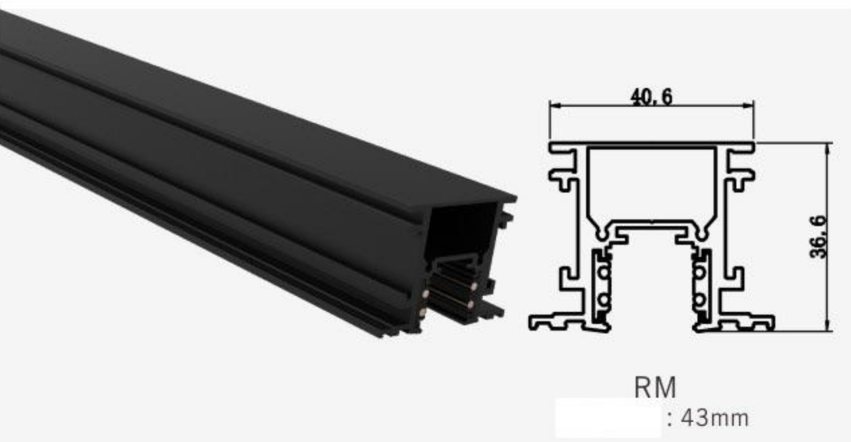
RM Size : 40.6X36.6X48.8
