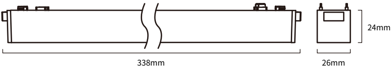
18T 18W 338x26x24mm
