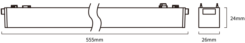
30T 30W 555x26x24mm
