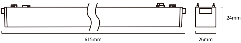
600F 20W 615x26x24mm
