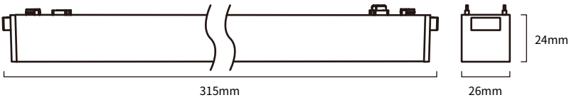
300F 10W 315x26x24mm
